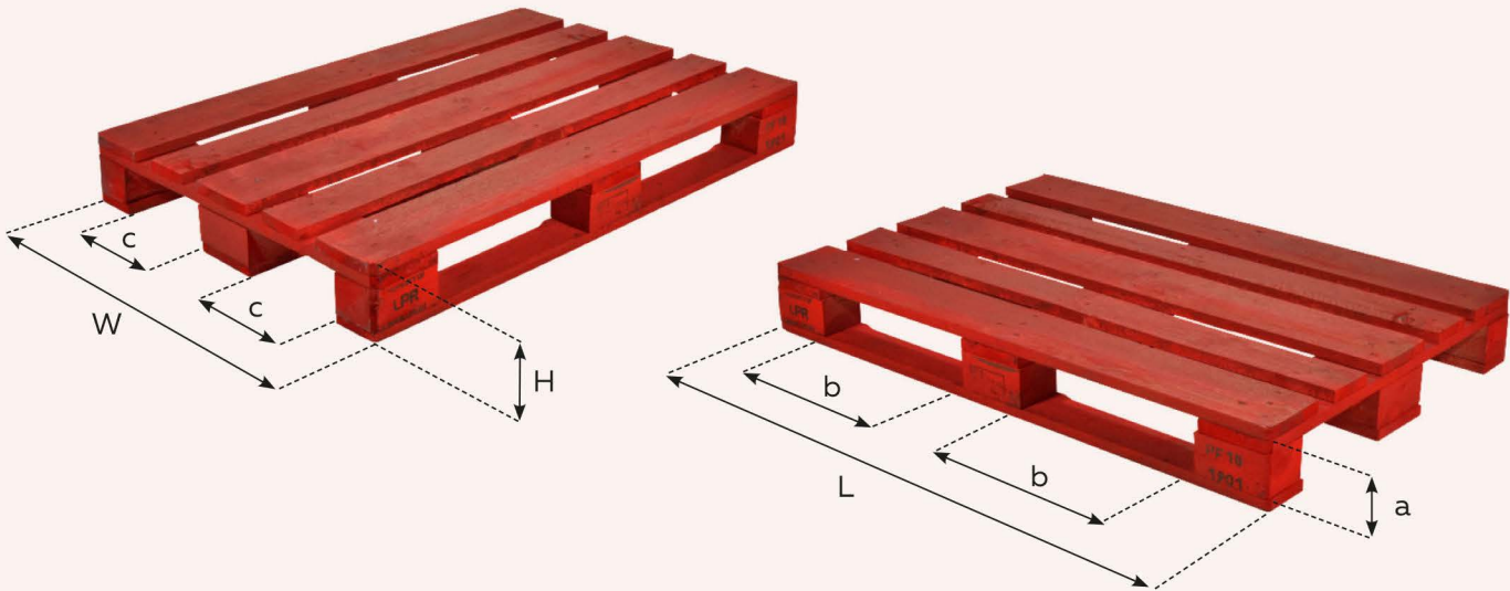
PRO80 - Pallet nominal dimensions & tolerance (mm)
